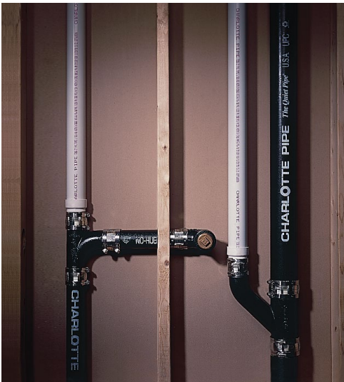
Cast iron risers, perfectly sized to work with our PVC pipe and fittings, provide an ultra-quiet plumbing system.
