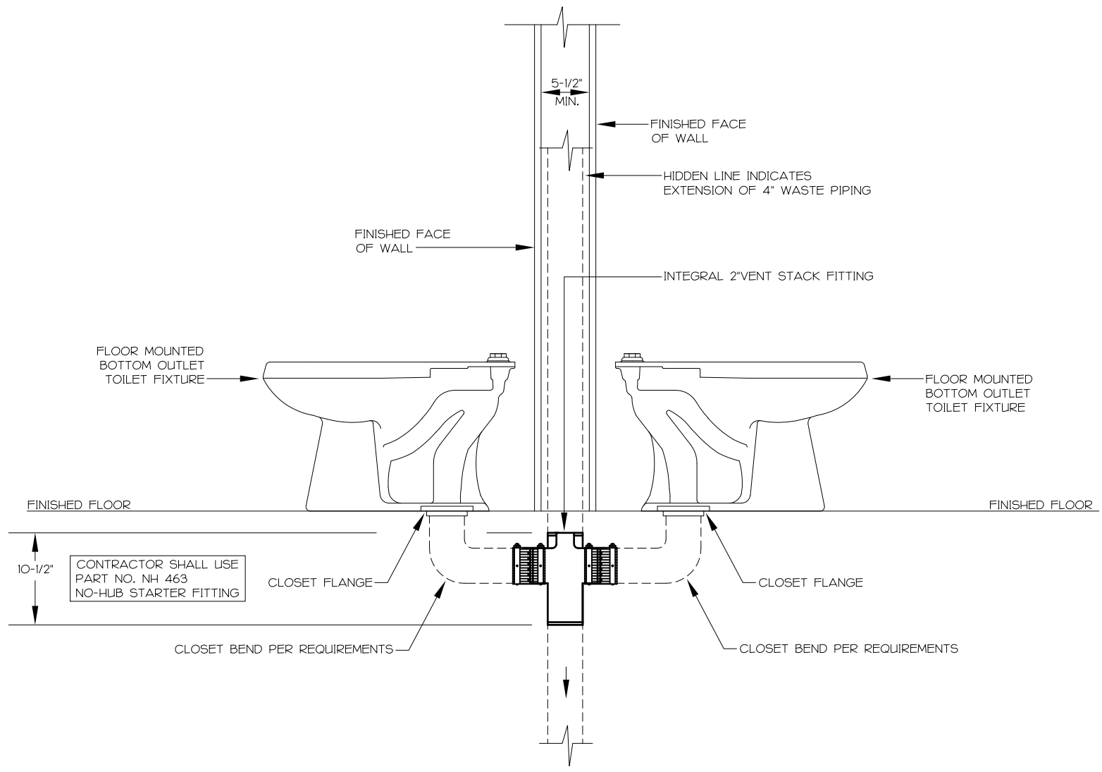
DOUBLE FITTING UNDER-SLAB - LEFT SIDE ELEVATION
