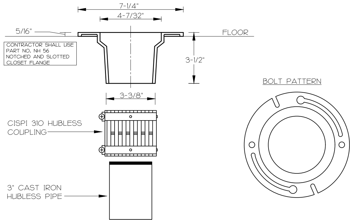
PART NO. NH 56 NOTCHED AND SLOTTED CLOSET FLANGE
