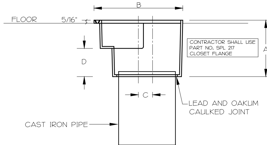
PART NO. 217 1"-2" OFFSET CLOSET FLANGE
