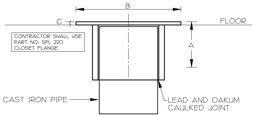
PART NO. SPL 220 CLOSET FLANGE, NOTCHED AND SLOTTED
