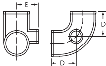
Edge HP Quarter Bend with 2" Side Inlet
