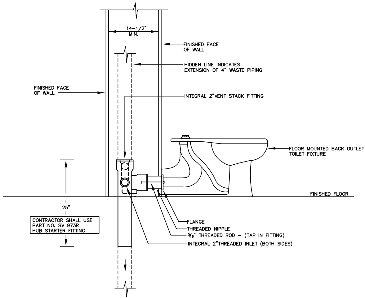
RIGHT HAND FITTING - LEFT SIDE ELEVATION
